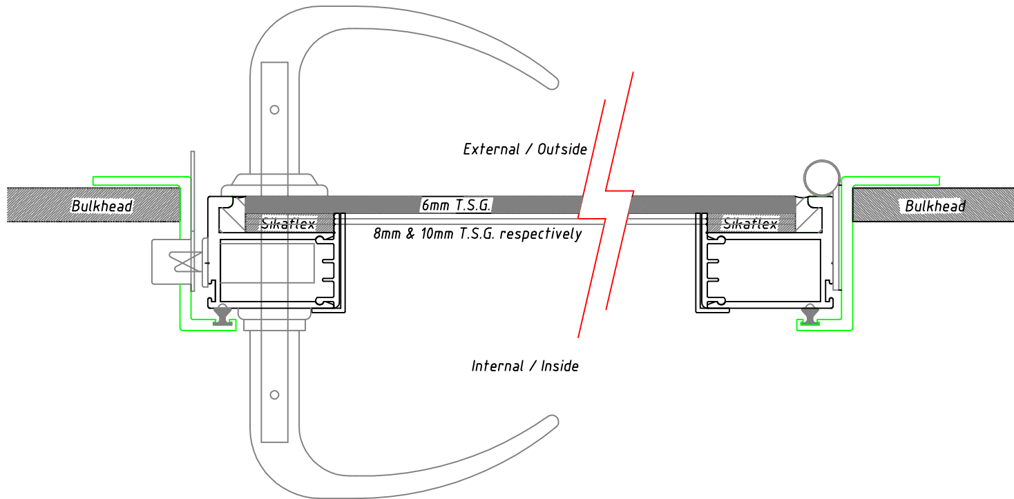
PLAN VIEW - DOOR SECTION
