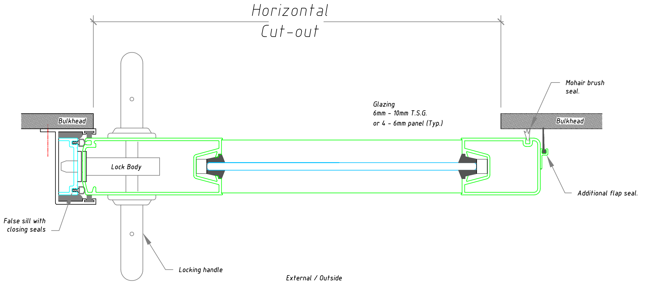
PLAN VIEW - HD SLIDING DOOR SECTION BULKHEAD MOUNT
